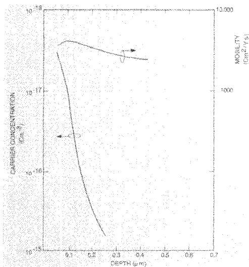
Figure 5. Ion Implanted Carrier Profile for the FET Active Layer
