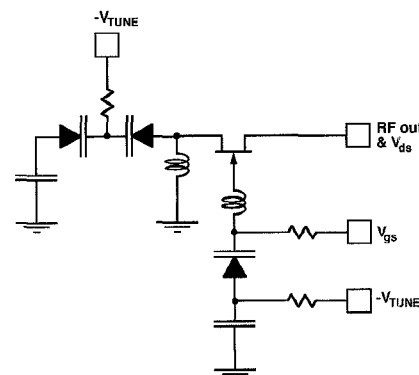
Figure 2. Typical VCO Schematic
