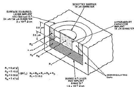
Figure 1. Cross-Section of the Planar Ion-Implanted Hyperabrupt Varactor Diode
