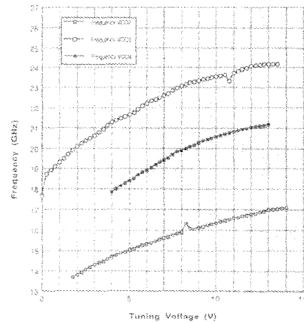
Figure 8. Frequency vs. Tuning Voltage for Three Different MMIC VCO Chips
